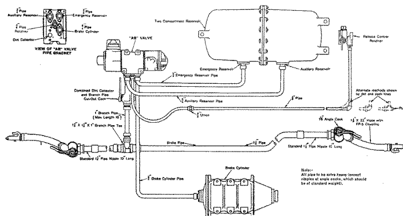
The “AB” Freight Brake Equipment – Instruction Pamphlet No. 5062 WestingHouse Air Brake Company, Dec. 1945
